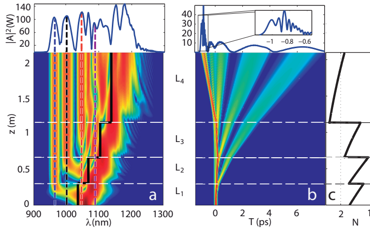
Fig. 3. (a) Spectral and (b) temporal evolution of an input pulse at \lambda_0 = 1060 nm with P_0 = 10 kW and a width of 65 fs (FWHM). The shifting \lambda_{zGV D} (initially at 1035 nm) is marked by the solid black line in (a) and the vertical dashed correspond to the \lambda_{Ch} predicted by Eq. (3): 958 (blue), 1002 (black), 1048 (red) and 1086 nm (magenta). (c) Evolution of the soliton order, N , for each fiber segment of length L_j . The value of N is approximately the same for both solitons resulting from fission by the end of the last segment, L_4 (both N(z) lines overlap).
