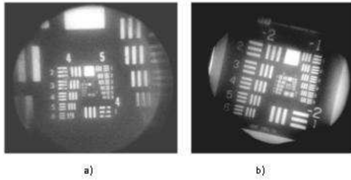
Fig. 3. Images given by an immersion oil lens. a) When object (a USAF test target) was 5 cm from the lens. b) When object was 56 cm from the lens.
